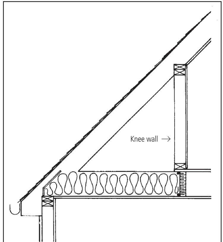
It is important to air seal under the knee wall.
