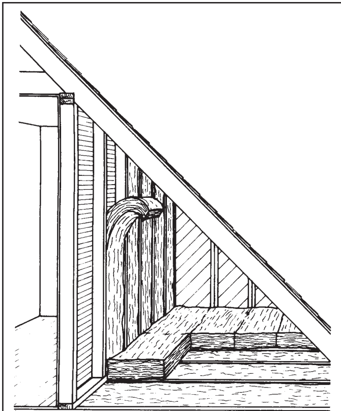
The wall and floor sections of a half storey should be insulated.
